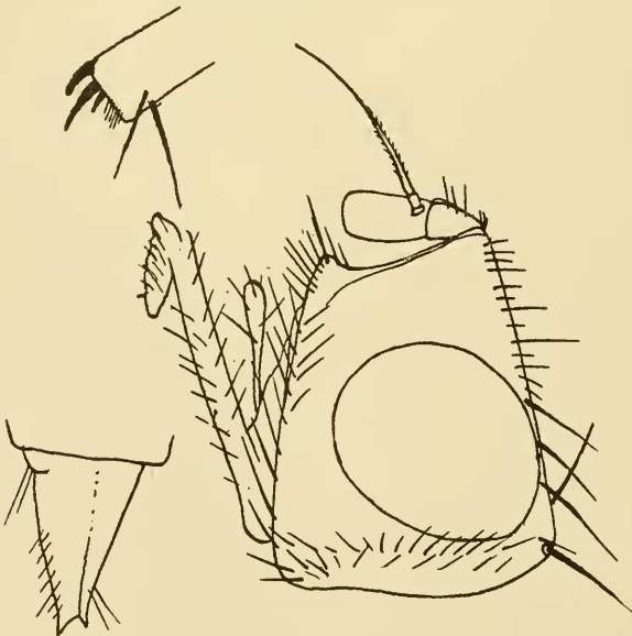
FIG. 1. Macateecia protuberans sp. n., female, head; apex of hind tibia, anterior view; and apex of abdomen, side view.
